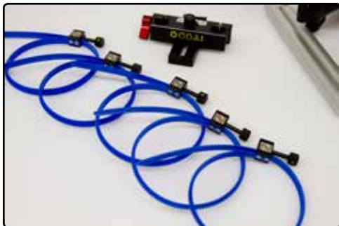
There are five gear rings for quick and easy lens changes. Also, the kit includes rail extensions and large lens support.
